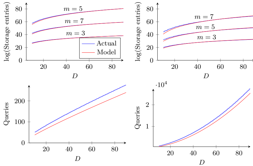
Fig. 1. Comparison of model and actual performance characteristics, assuming q = 2^{20} , \|f\|_\infty = q/2 , and N = \binom{D+m}{m} for Algorithm 2 (left) and Algorithm 3 (right). As the required storage size also depends on the number of variables m of the polynomial, we include plots for different values of m . Actual performance was computed with a SAGE script using the smallest possible values for r .
